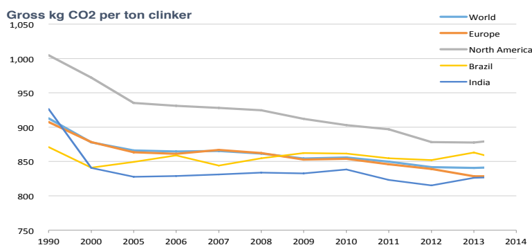
Figure 6 - Gross kg CO 2 per ton clinker source: CSI Getting the Numbers (GNR) database ( www.wbcsdcement.org/GNR )
