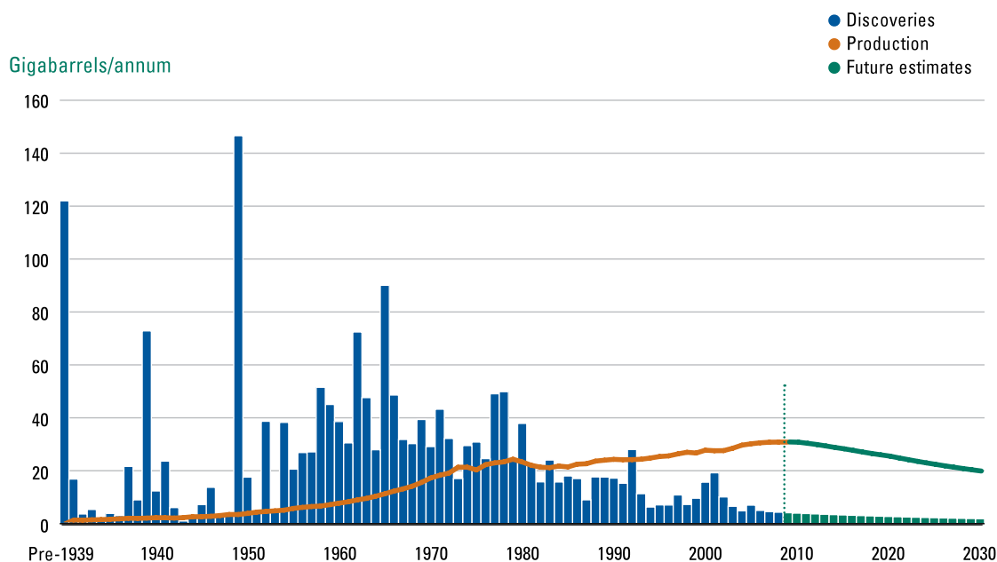
Figure 2.10. World conventional oil discoveries and production
