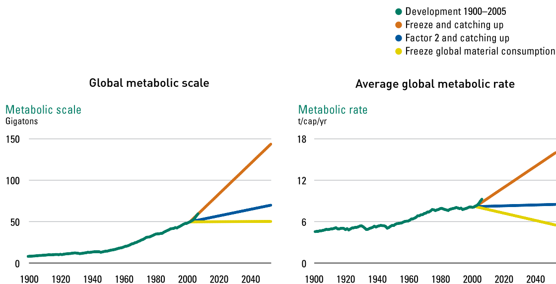
Figure 2.15. Resource use according to three different scenarios up to 2050
