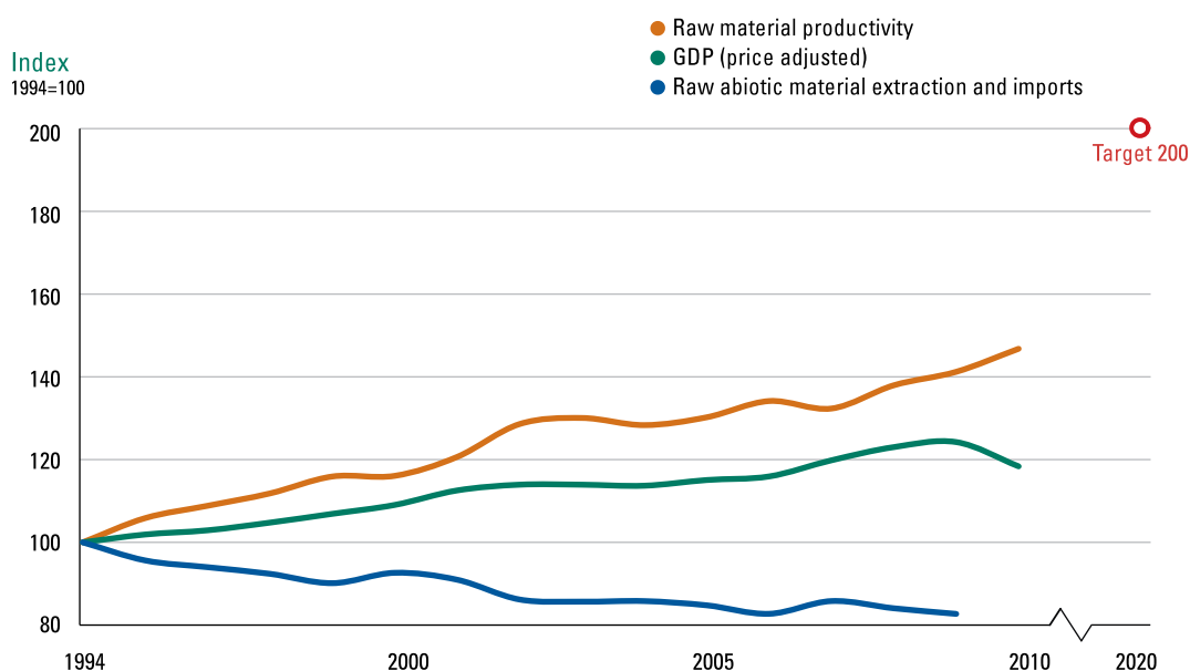
Figure 6.1. Resource productivity and GDP growth
